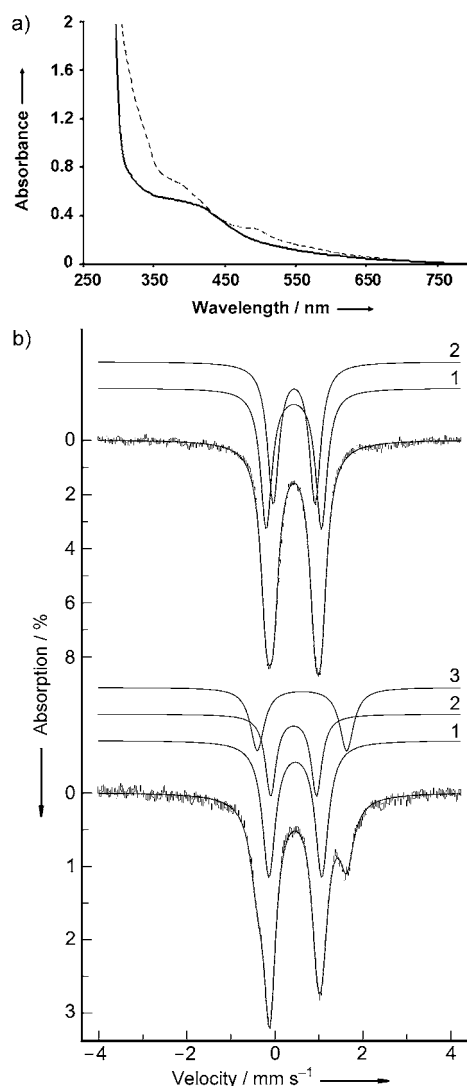
Figure 2. a) UV/Vis spectrum of 57 Fe/S-NadA (300 μM) in Tris-HCl (100 mM, pH 7.5), NaCl (50 mM) without (—) or with (---) DTHPA (1.8 mM). b) Mössbauer spectra of 57 Fe/S-NadA in the absence (top) and in the presence (bottom) of DTHPA (6 equiv). Taken at 4.2 K with an external magnetic field of 0.06 T applied parallel to γ rays. Traces 1, 2, and 3 represent component contributions (see text for details).
